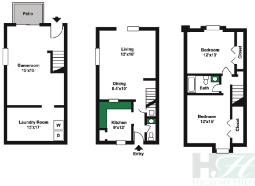
1550 Sq. Ft. 2 Bedroom Townhome with Gameroom & Fireplace
